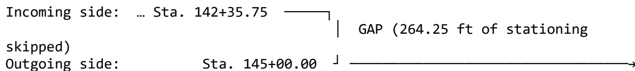
Figure 9.3.2-1 — Station gap equation. Geometry is continuous; station numbers jump forward.
