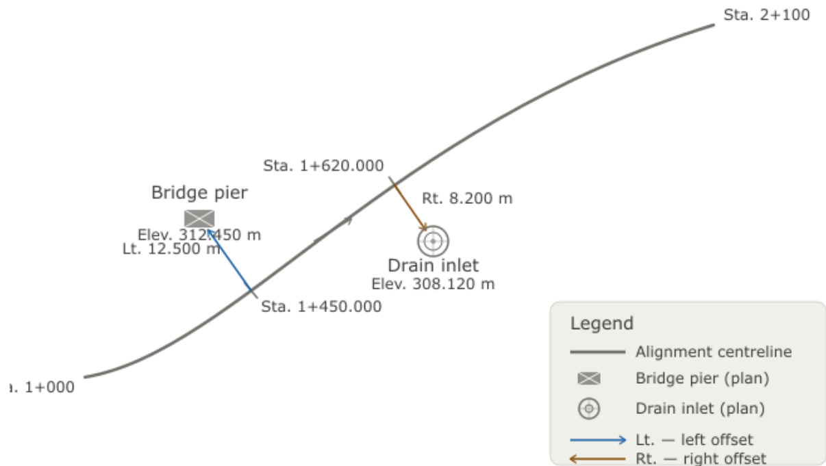
Figure 8.1.2-1 — Conceptual diagram showing a plan view of an alignment with a bridge pier placed at a station/offset and a drain inlet placed at station/offset/elevation.
