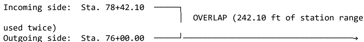
Figure 9.3.3-1 — Station overlap equation. Geometry is continuous; station numbers jump backward.
