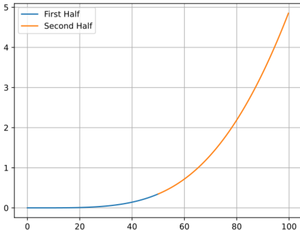
Figure 2.7.2-3 - Final Helmert transition curve
