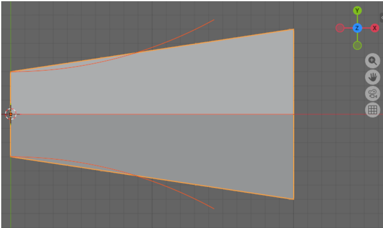
Figure 10.6.1.6-1 — Plan view of IfcSectionedSurface_with_stringlines_independent_edge_alignments.ifc . The centerline (Main-Line) and arc edge alignments (Left_Edge, Right_Edge) are shown; the surface geometry between them is indeterminate due to the specification gaps described above.
