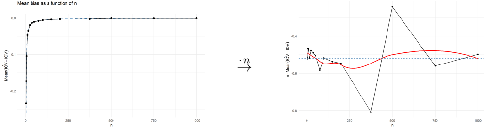
Figure 4.4.: Left: Mean from simulation (solid) and theoretical approximation (dashed) of (\widehat{\text{IOV}} - \text{IOV}) . Right: the same quantities rescaled by a factor of n . For n \in N_{\text{fine}} and Scenario B with \pi = 0.75 . Based on B = 20,000 replications.
