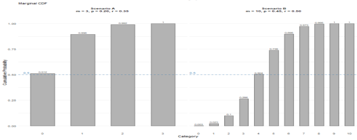
Figure 4.1.: Marginal CDFS of the two simulation scenarios.
