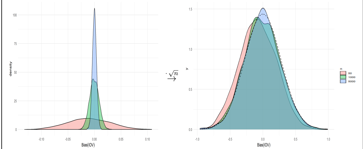
Figure 4.3.: Left: simulated density of (\widehat{\text{IOV}} - \text{IOV}) for n \in \{50, 1000, 5000\} . Right: the same quantity rescaled by a factor of \sqrt{n} , i.e. \sqrt{n}(\widehat{\text{IOV}} - \text{IOV}) , overlaid with the asymptotic \mathcal{N}(0, \sigma_{\text{IOV}}^2) limit (dashed). Scenario B with \pi = 0.75 . Based on B = 1,000 replications.
