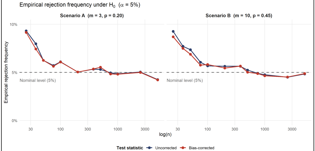
Figure 4.9.: Rejection rates of \hat{\kappa}_{\text{ord}}(1) and \hat{\kappa}_{\text{ord}}^{\text{bc}}(1) for both scenarios under H_0 (i.e. r = 0 ), across n \in \{25, 37, 50, 75, 100, 200, 375, 500, 750, 1000, 2500, 5000\} , using a nominal significance level of \alpha = 5\% for B = 5000 iterations.
