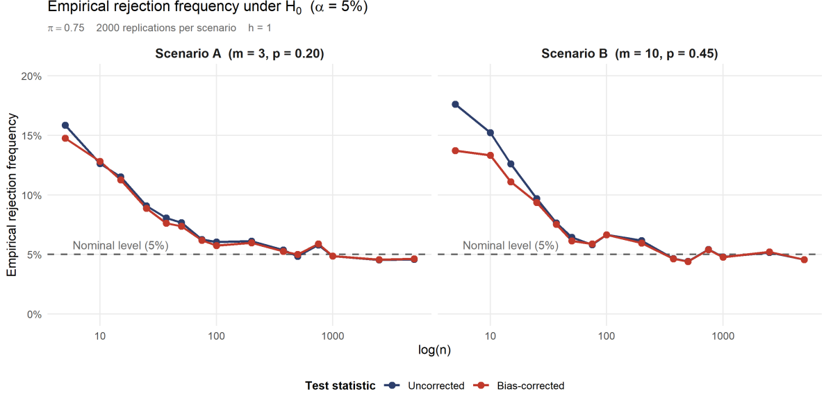
Figure 4.8.: Rejection rates of \hat{\kappa}_{\text{ord}}(1) and \hat{\kappa}_{\text{ord}}^{\text{bc}}(1) for both scenarios under H_0 (i.e. r = 0 ), across n \in \{5, 10, 15, 25, 37, 50, 75, 100, 200, 375, 500, 750, 1000, 2500, 5000\} , using a nominal significance level of \alpha = 5\% .
