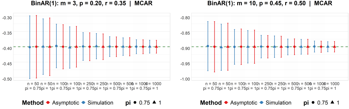
Figure 4.6.: Simulated vs. asymptotic standard deviation of \widehat{\text{skew}} for Scenario B ( m = 10, p = 0.45, r = 0.50 ) across n \in \{50, 100, 250, 500, 1000\} and \pi \in \{0.75, 1\} .
