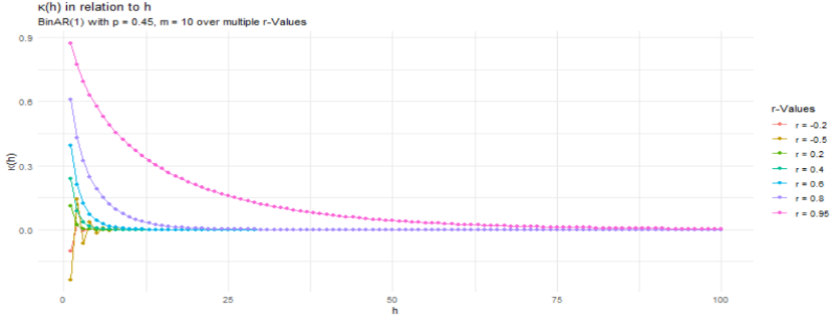
Figure 4.1.: Cohen's \kappa_{\text{ord}}(h) for different values of r .
