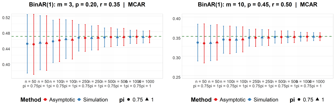
Figure 4.5.: Simulated vs. asymptotic standard deviation of \widehat{\text{IOV}} for Scenario B ( m = 10 , p = 0.45 , r = 0.50 ) across n \in \{50, 100, 250, 500, 1000\} and \pi \in \{0.75, 1\} .
