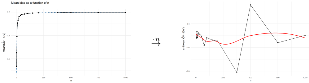
Figure 4.4.: Left: Mean from simulation (solid) and theoretical approximation (dashed) of (\widehat{\text{IOV}} - \text{IOV}) . Right: the same quantities rescaled by a factor of n . For n \in \{2, 3, 5, 10, 15, 25, 37, 50, 75, 100, 150, 200, 375, 500, 750, 1000\} and Scenario B with \pi = 0.75 . Based on B = 20,000 replications.
