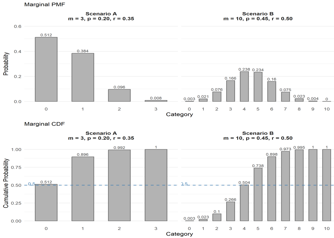
Figure 4.2.: Marginal distribution of the two simulation scenarios.
