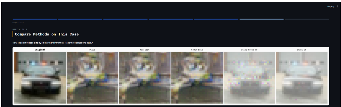
Figure 35: Compare methods 1.1
