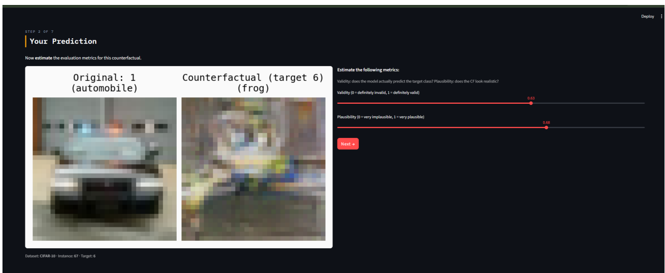
Figure 31: User Prediction
