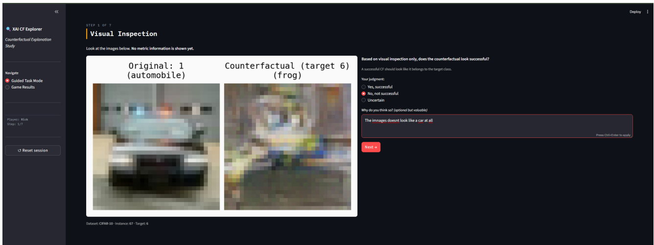
Figure 30: Visual Inspection
