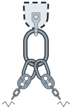
DETAIL A — HEAD OF SLING 1:10
