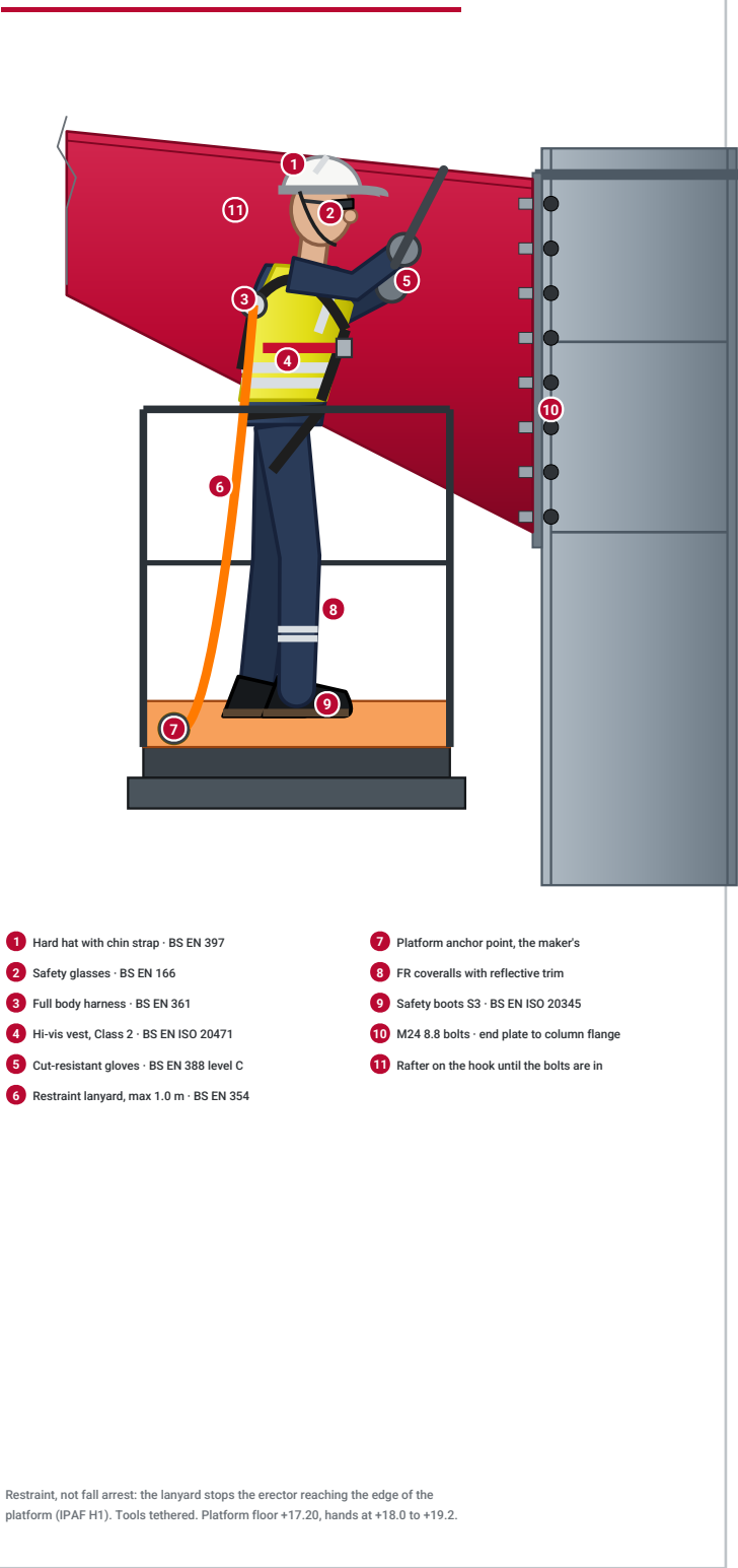
DETAIL C – CONNECTING AT THE VALLEY COLUMN · 1:25
