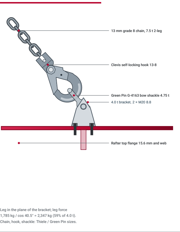
DETAIL D – KIT C LIFTING POINT · 1:10
