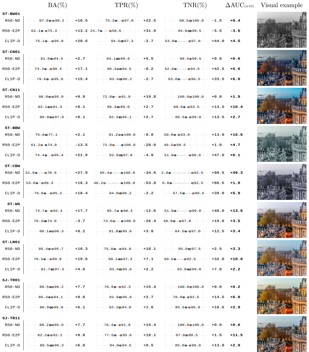
Figure 6: Performance of the standard (blue) and adapted (orange) detectors on the investigated presets for the PRE data.
