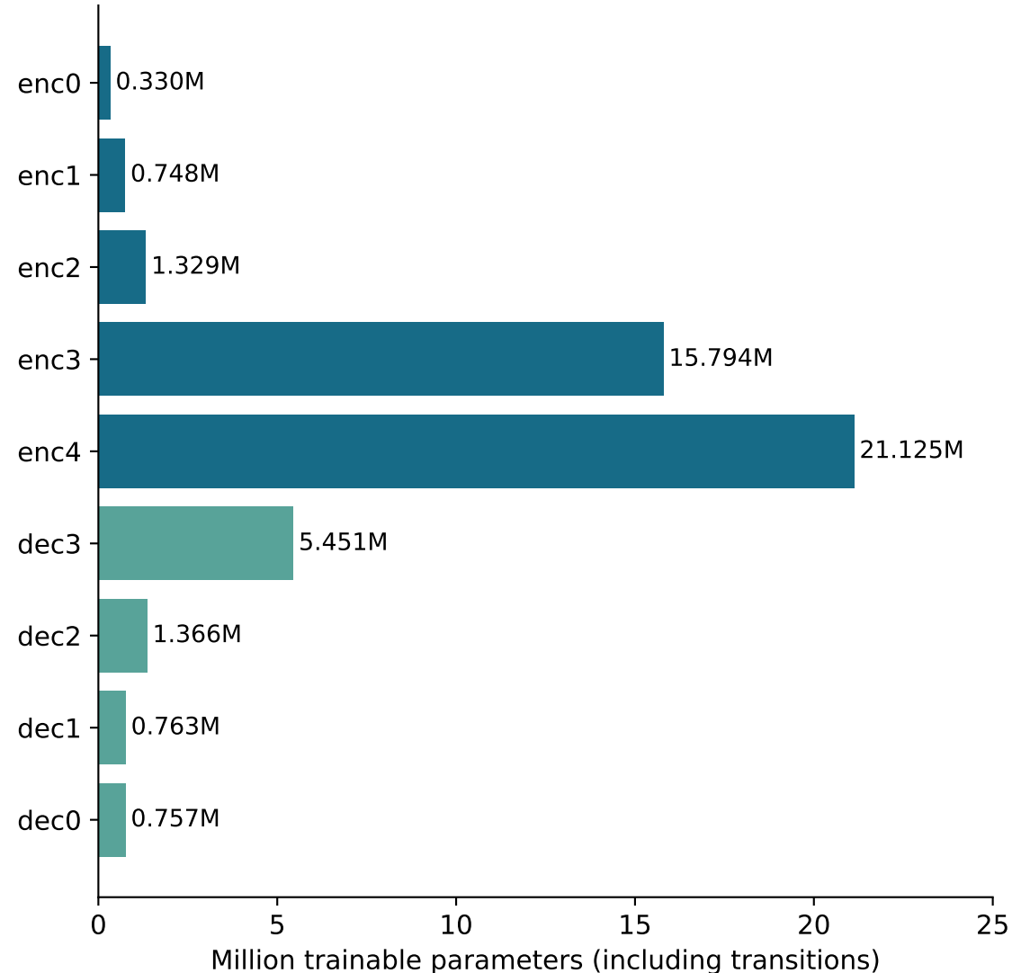
Parameters by U-Net stage
