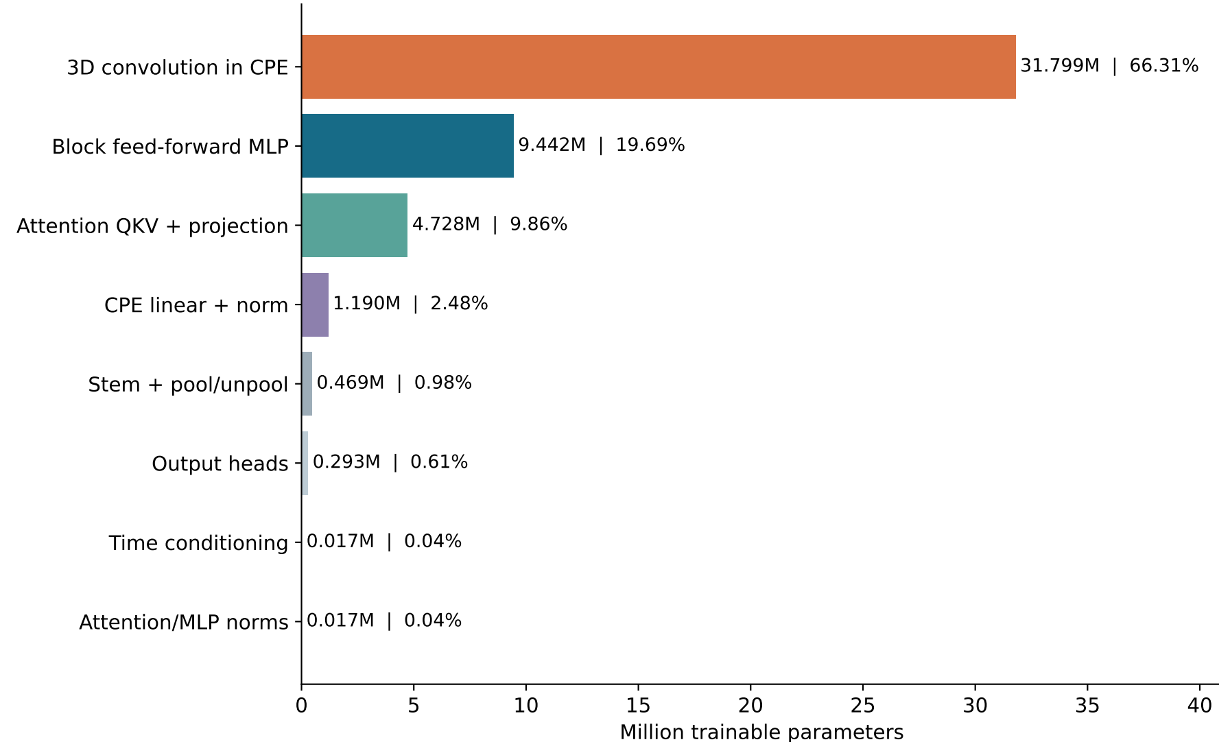
Where the 47.956M parameters go
