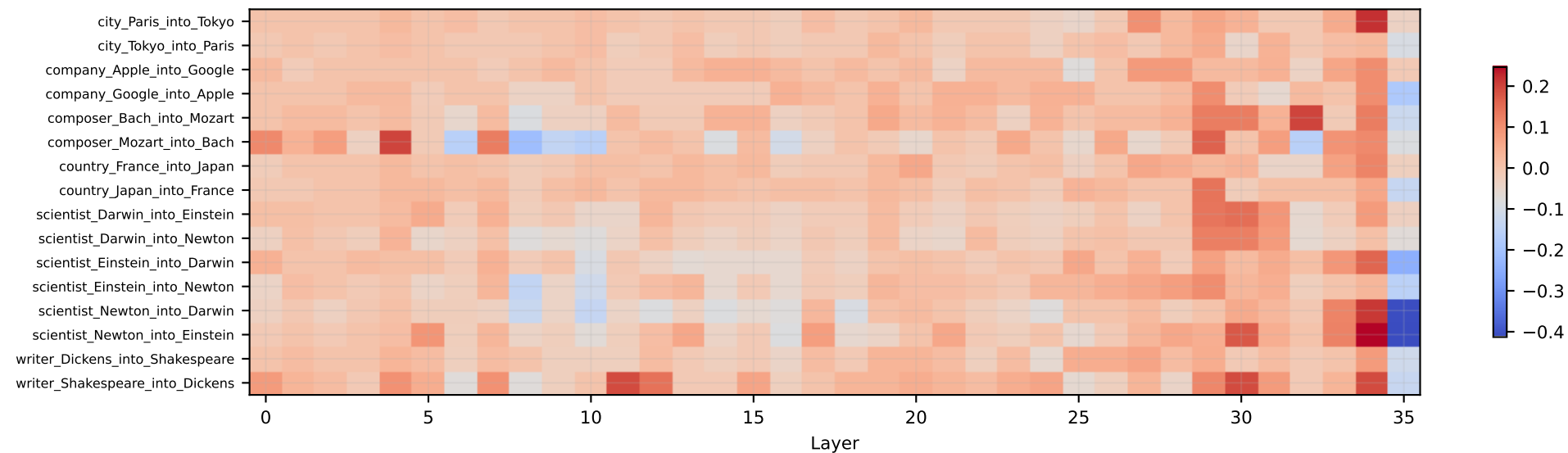
MLP effect P10
