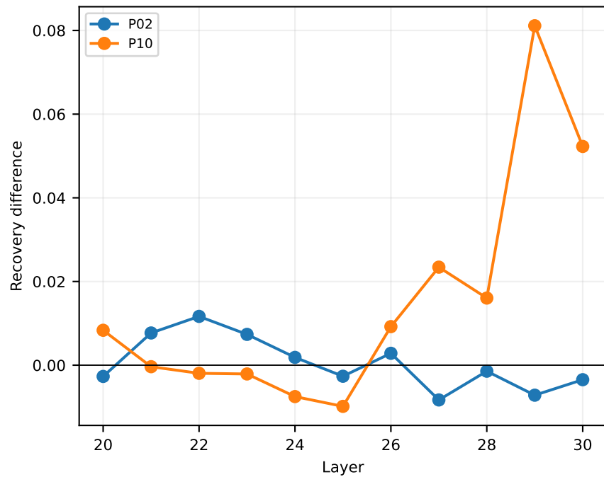
MLP active – bypass
