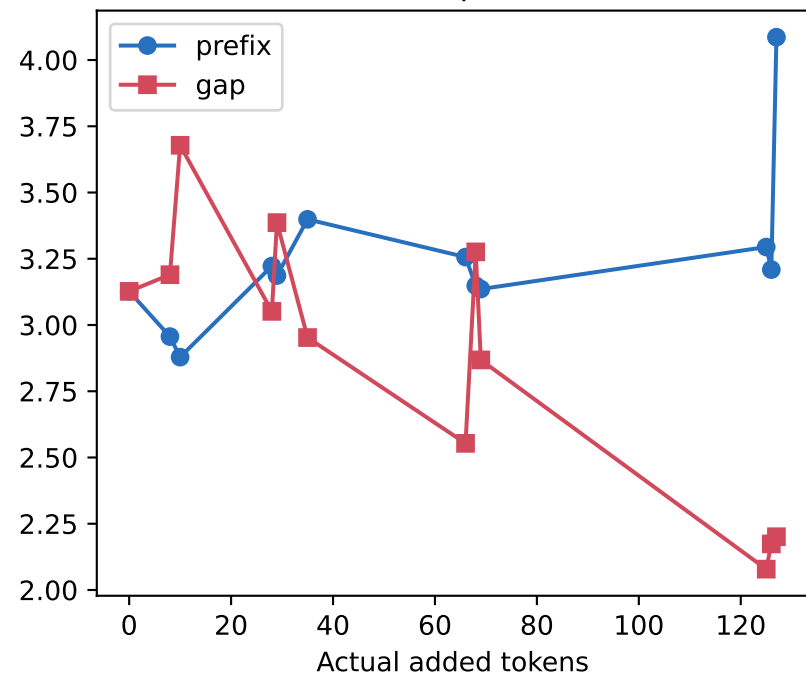
Intermediate-position AUC
