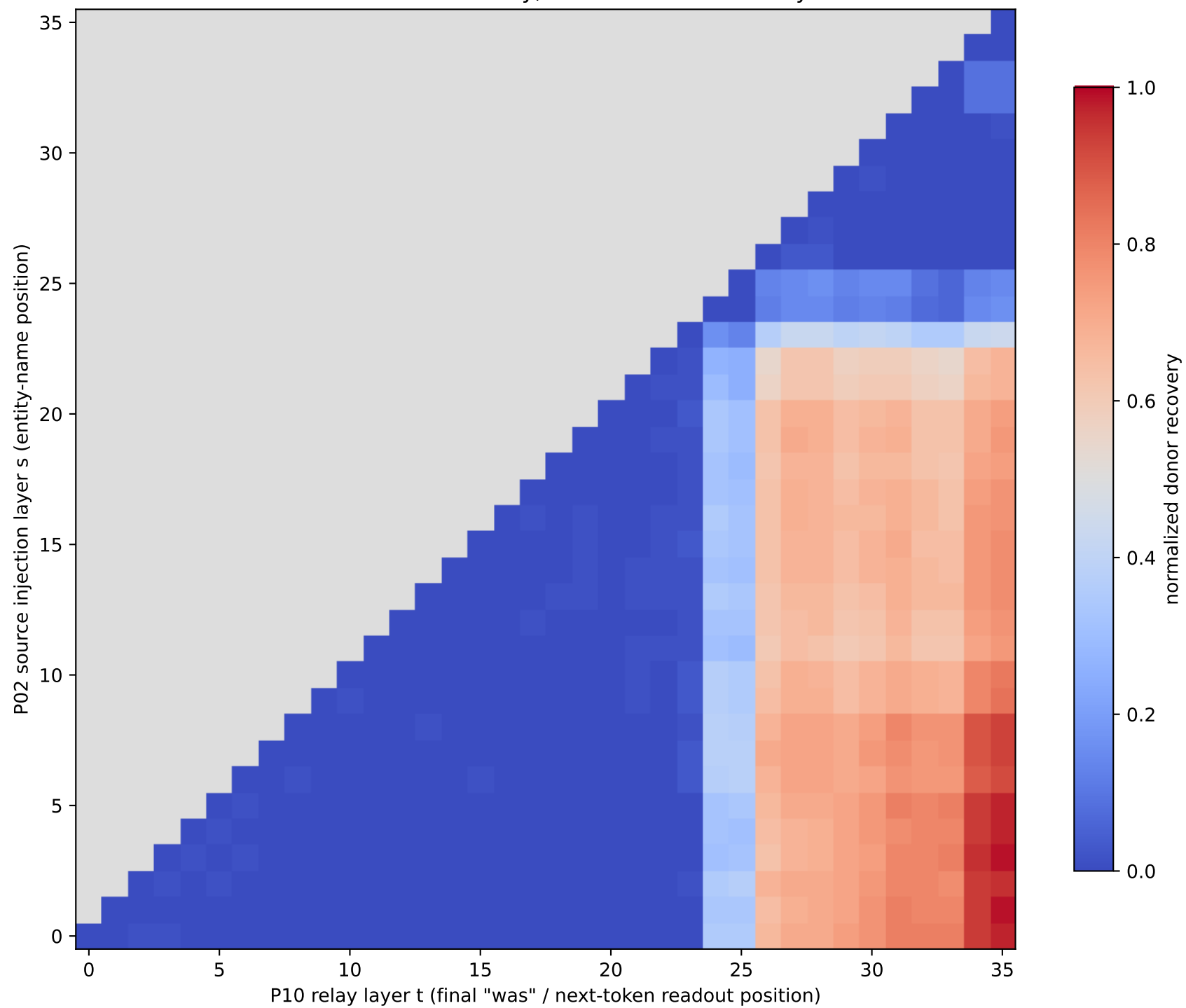
P10 relay for scientist_Newton_into_Einstein 0 = no donor recovery; 1 = full donor recovery
