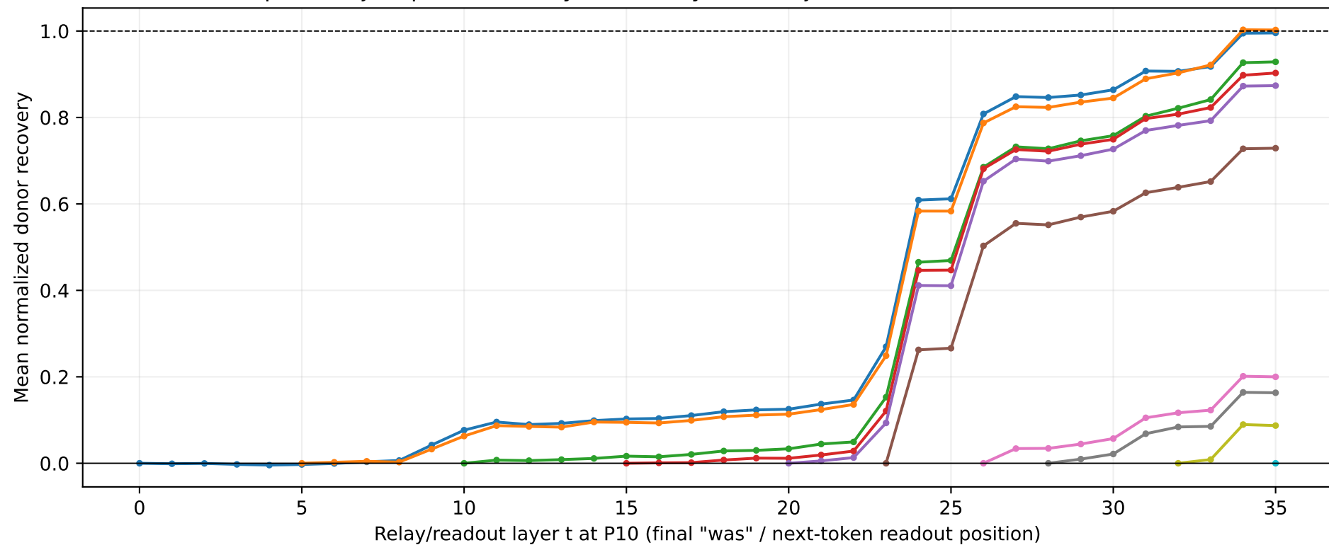
All post-subject positions relay: P02 entity-name injection to P10 final `was` readout
