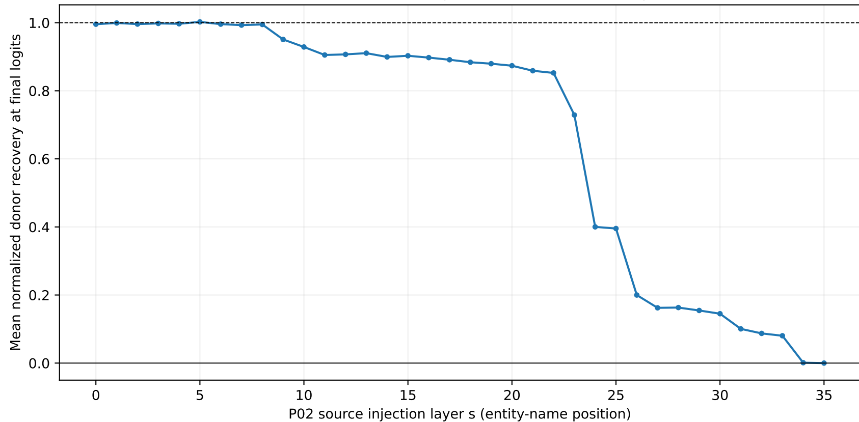
Source patch end-to-end: P02 entity name to P10 final "was" readout 0 = no donor recovery; 1 = full donor recovery
