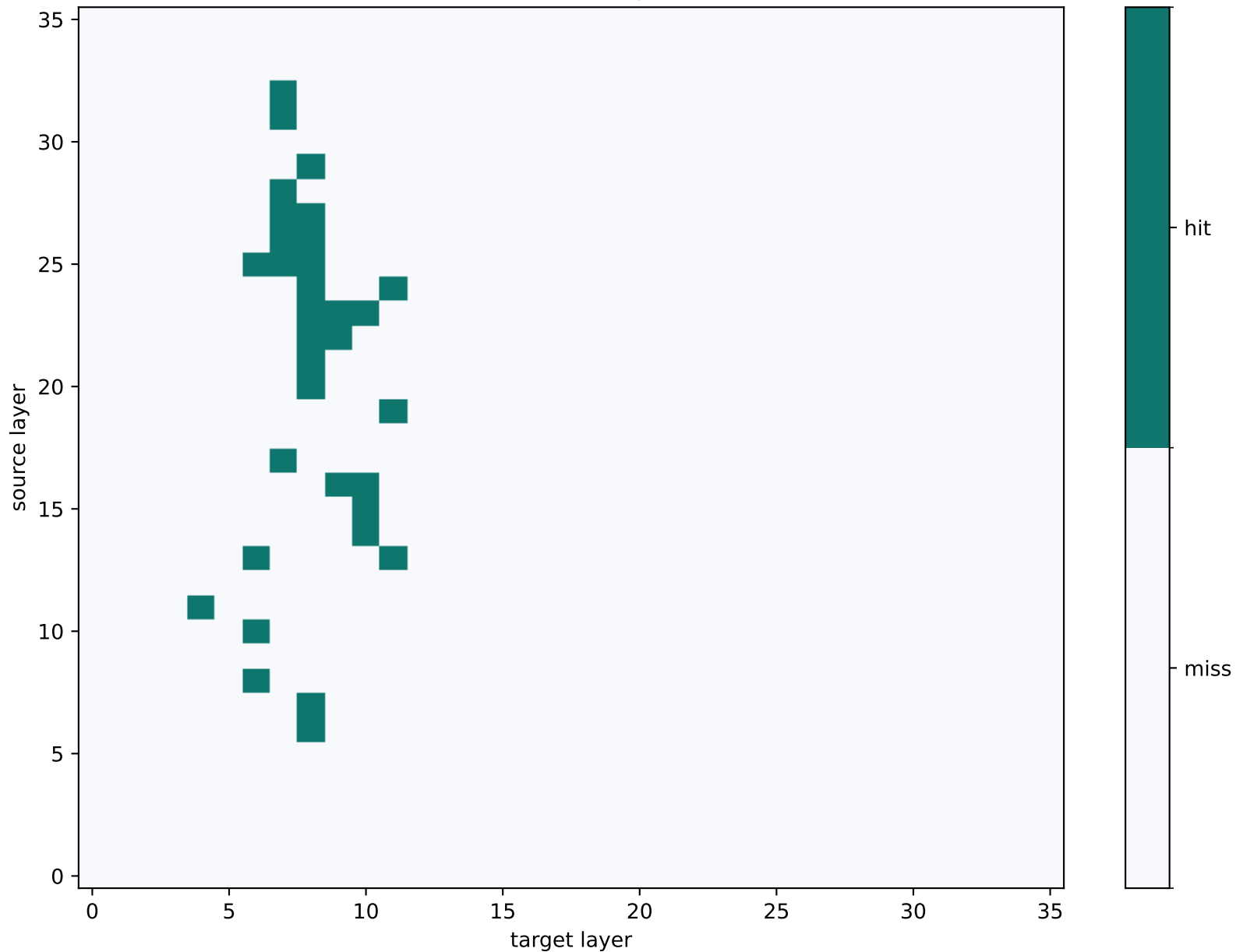
x refers to Diana, princess of Wales | hits 33/1296
