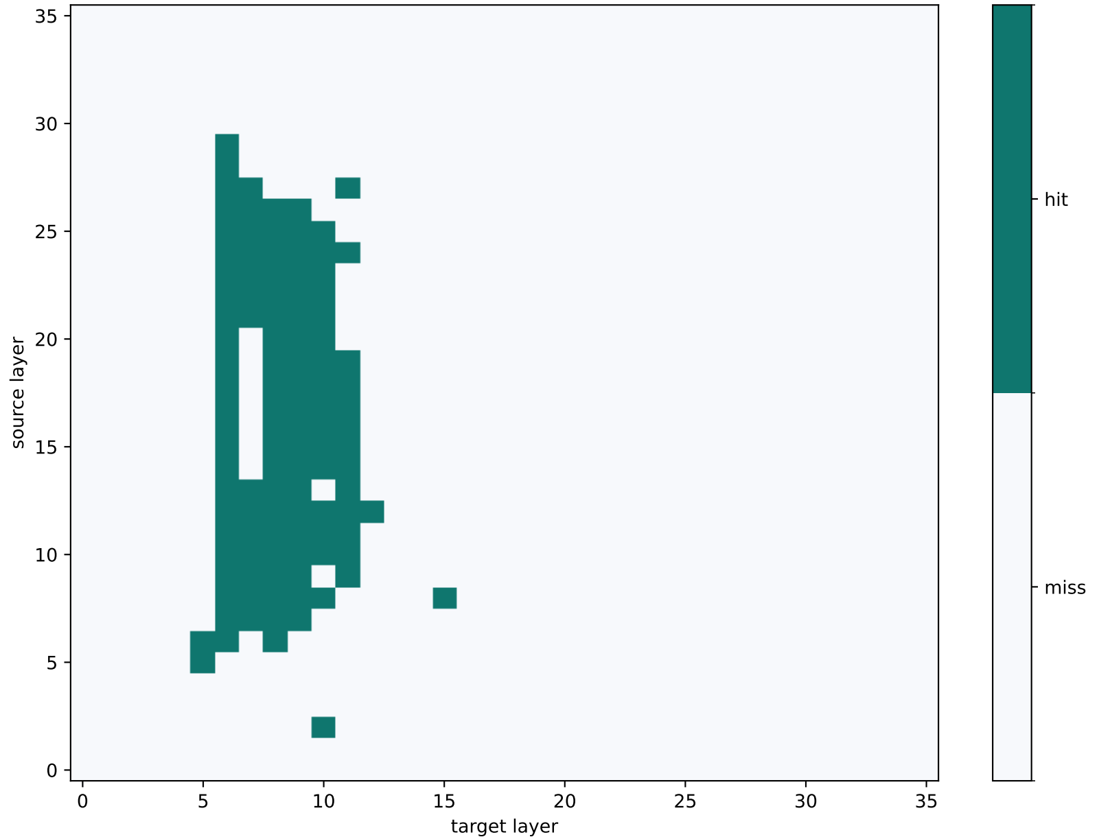
x was Alexander the Great | hits 113/1296
