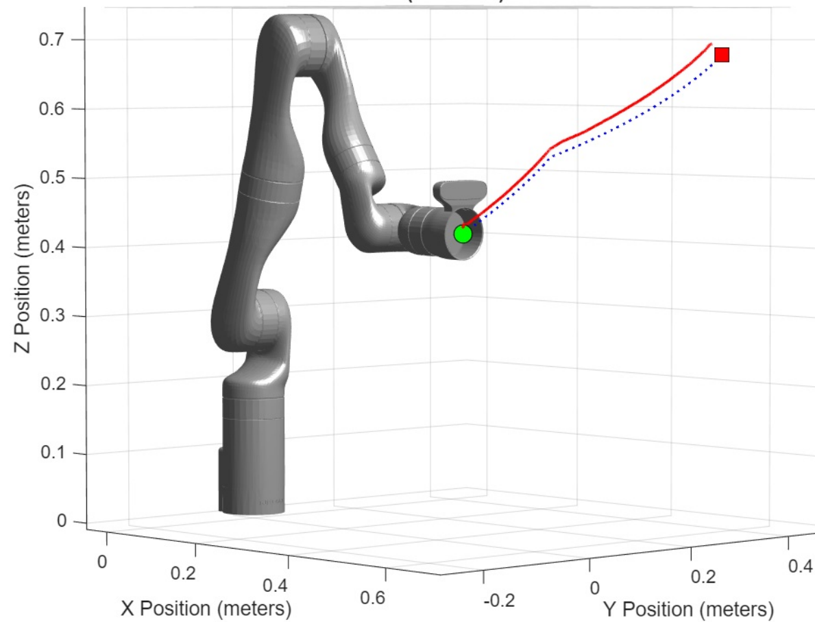
Confident Kinova Gen3 7-DOF: Designed vs Tracked Trajectory ( t = 0.00 s)
