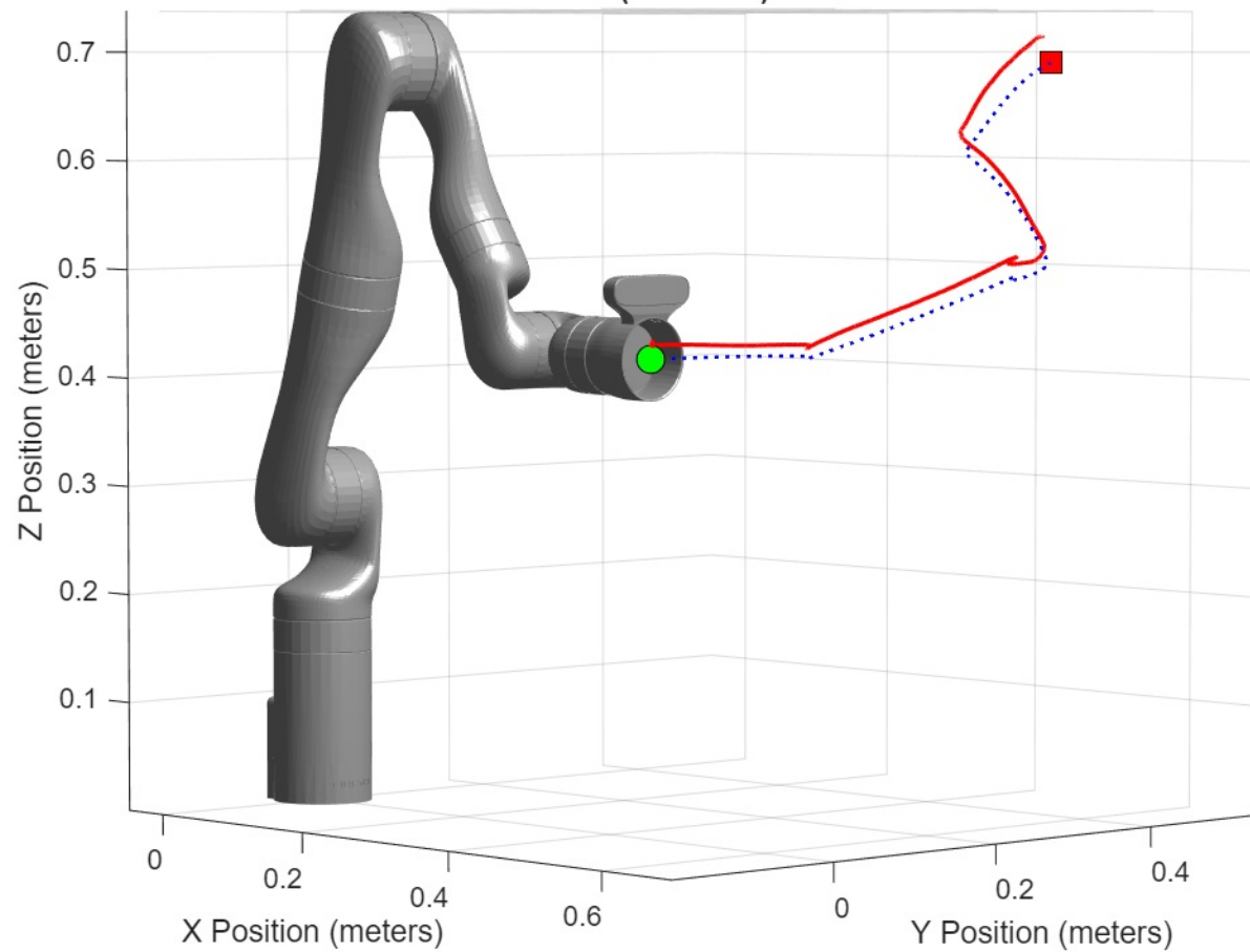
Curious Kinova Gen3 7-DOF: Designed vs Tracked Trajectory ( t = 0.00 s)
