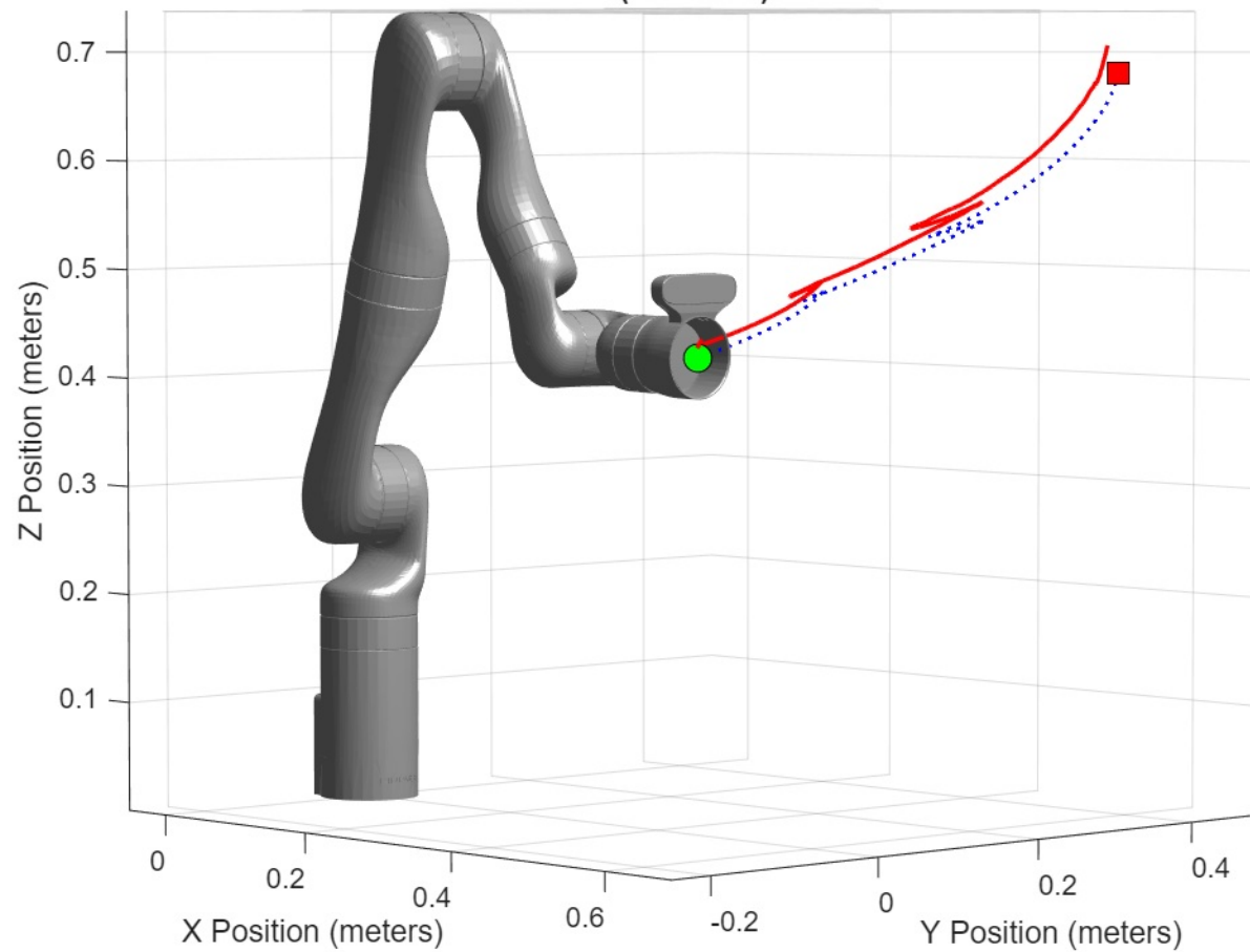
Fearful Kinova Gen3 7-DOF: Designed vs Tracked Trajectory ( t = 0.00 s)
