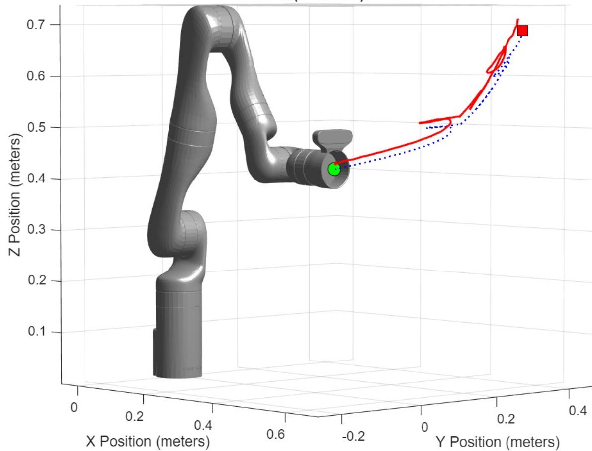
Hesitant Kinova Gen3 7-DOF: Designed vs Tracked Trajectory (t = 0.00 s)
