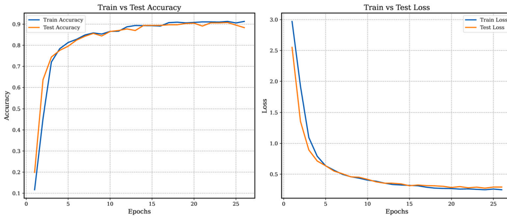
Fig. 20. Accuracy and loss vs. epochs of the applied CNN-LSTM model.
