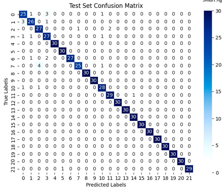
Fig. 16. Confusion matrix of the stacked ensemble model.
