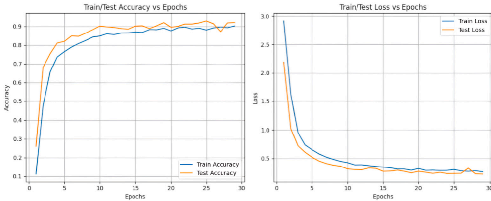
Fig. 19. Accuracy and loss vs. epochs of the applied LSTM model.
