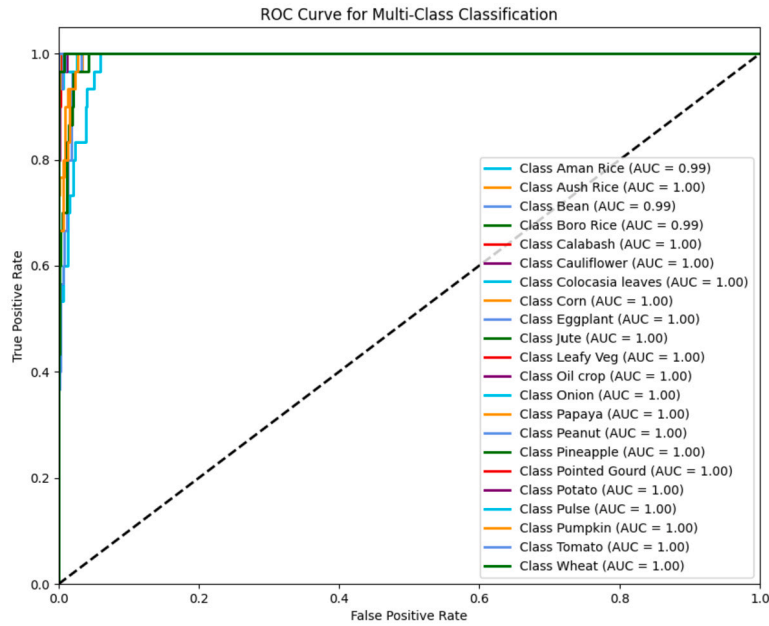
Fig. 22. ROC curve of the applied TabNet model.
