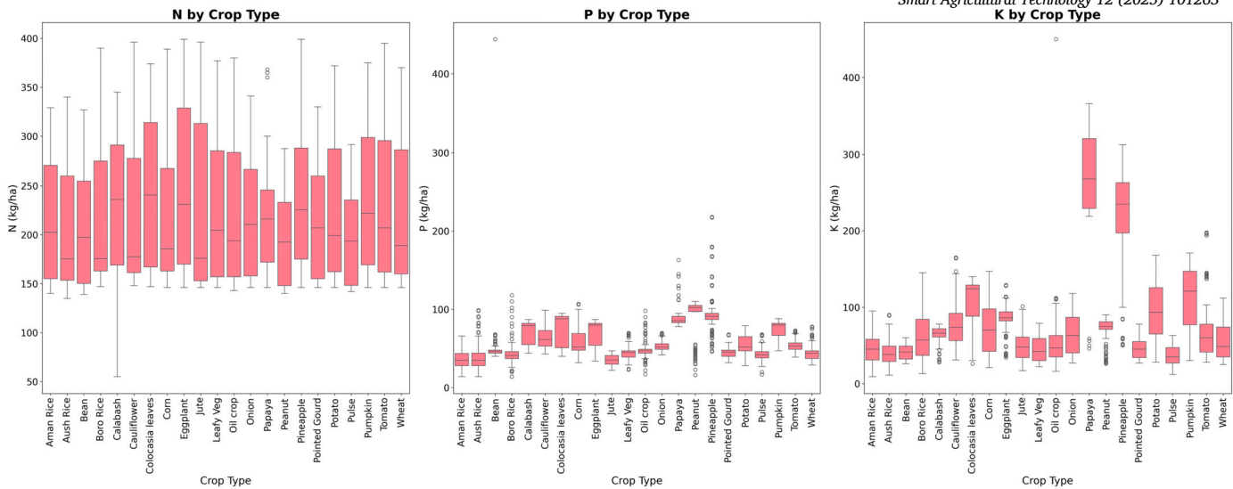
Fig. 3. NPK boxplots of the employed crop prediction dataset.
