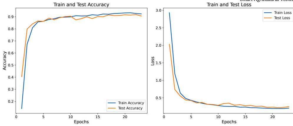
Fig. 21. Accuracy and loss vs. epochs of the applied CNN-BiLSTM model.
