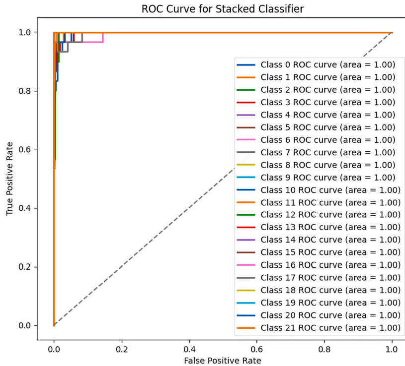
Fig. 15. ROC curve of the stacked ensemble model.
