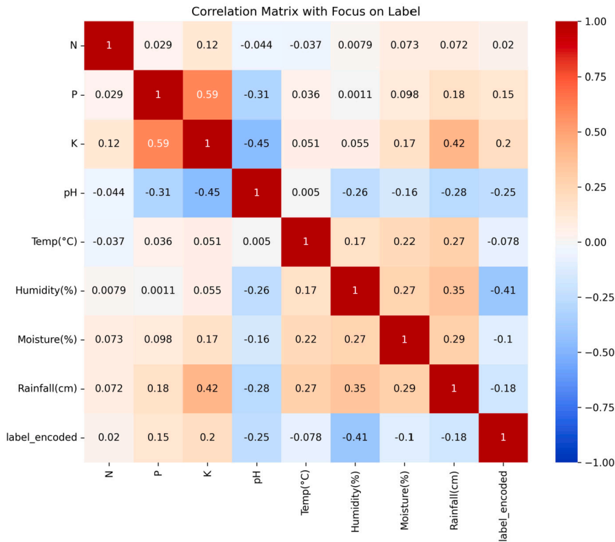
Fig. 7. Correlation heat map of various features of the employed crop prediction dataset.
