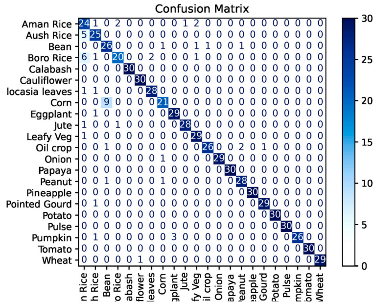
Fig. 23. Confusion matrix of the TabNet model.
