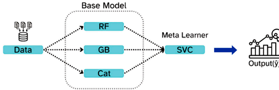
Fig. 14. Proposed SVC meta learner-based stacking architecture.
