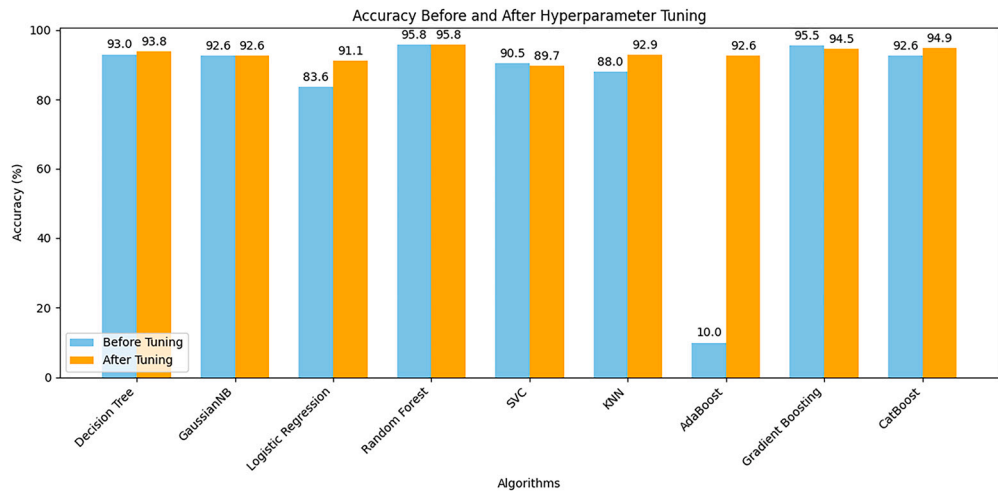
Fig. 13. Accuracies of the applied models with and without hyperparameter tuning.
