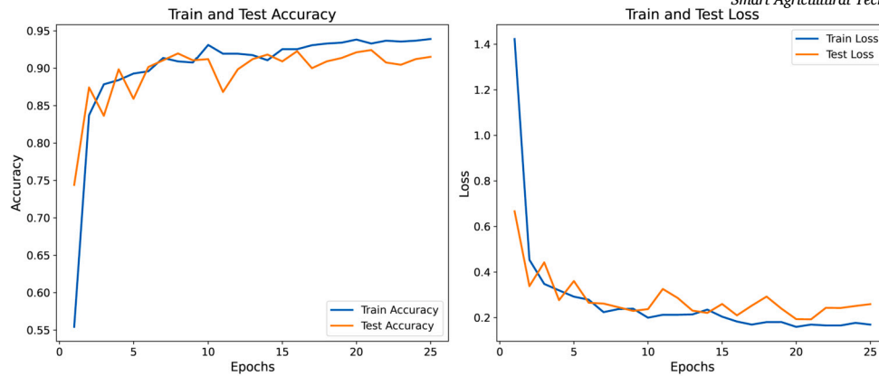
Fig. 18. Accuracy and loss vs. epochs of the applied CNN model.
