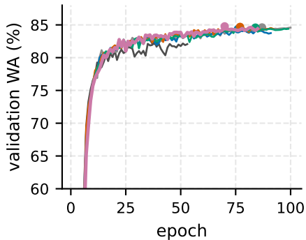
(a) validation WA, best epoch marked
