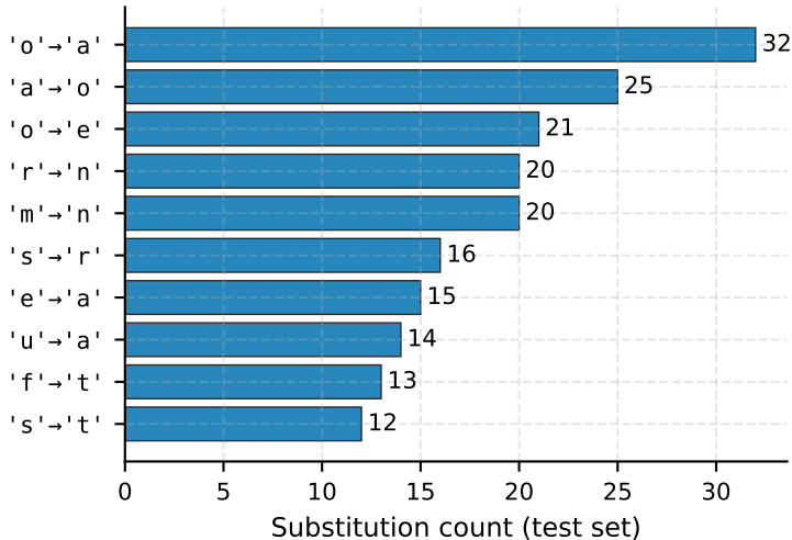
Top-10 character substitutions (AugCRNN-T)
