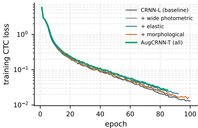
(b) training loss
