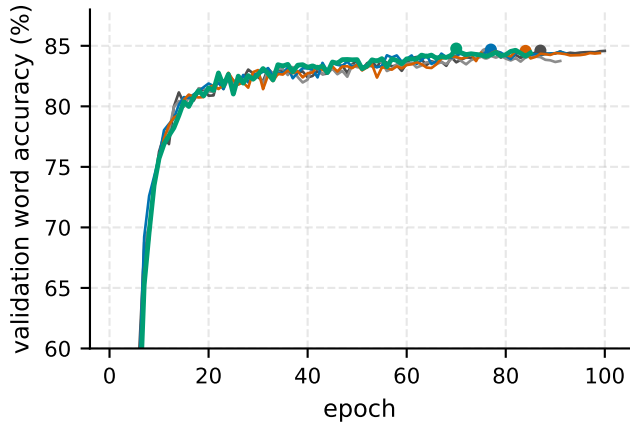
(a) validation WA, best epoch marked
