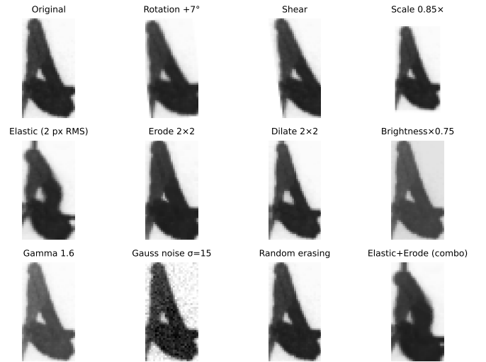
Fig. 2. Augmentation transforms on a training crop. The elastic panel uses the corrected amplitude (2 px RMS); the last panel shows the compound elastic+morphological effect.
