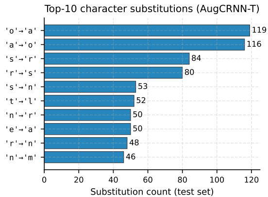
Fig. 4. Ten most frequent character substitutions of AugCRNN-T on the test set (true → predicted).
