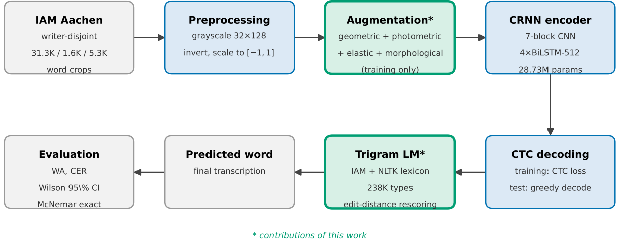
Fig. 1. Overview of AugCRNN-T. Word crops are normalised, augmented (training only), encoded by a CRNN and decoded with CTC; the decoded string is then corrected against a lexicon-extended n -gram language model (LM). Green boxes mark the two stages varied in the ablations. The evaluation stage reports word accuracy (WA), character error rate (CER) and Wilson confidence intervals (CI), all defined formally in Section IV.
