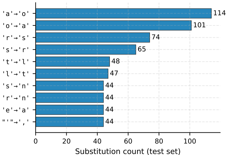
Top-10 character substitutions (CRNN-LX)
