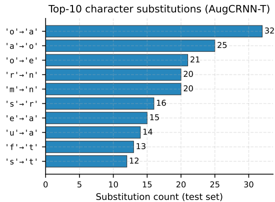
Fig. 4. Ten most frequent character substitutions of AugCRNN-T (true → predicted).
