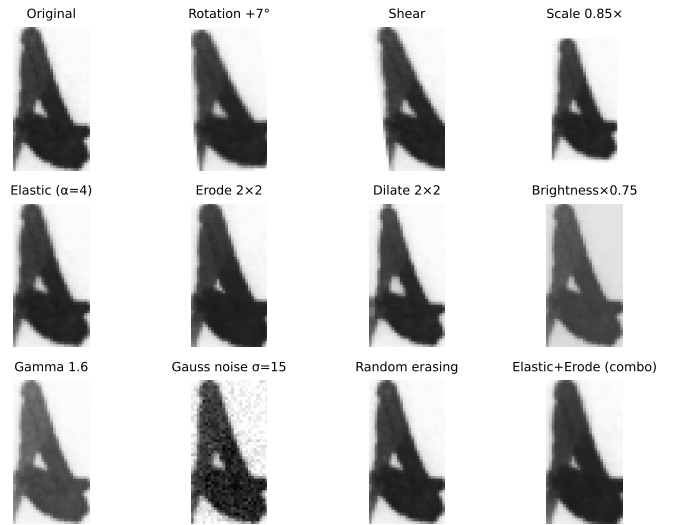
Fig. 2. Augmentation transforms on a training word. The last panel shows the compound elastic+morphological effect.
