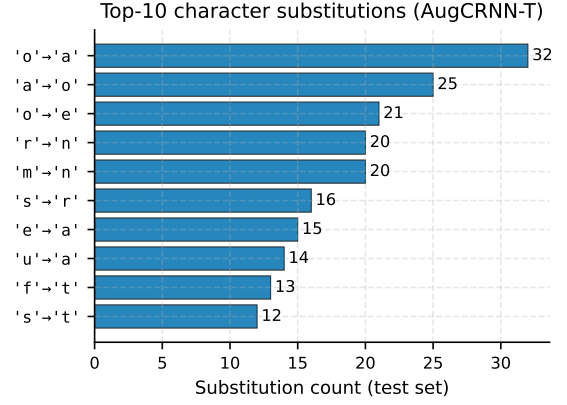
Fig. 4. Ten most frequent character substitutions of AugCRNN-T (true → predicted).
