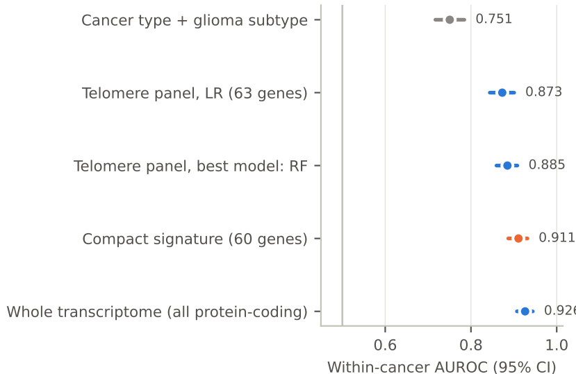
ALT, gliomas + sarcomas
