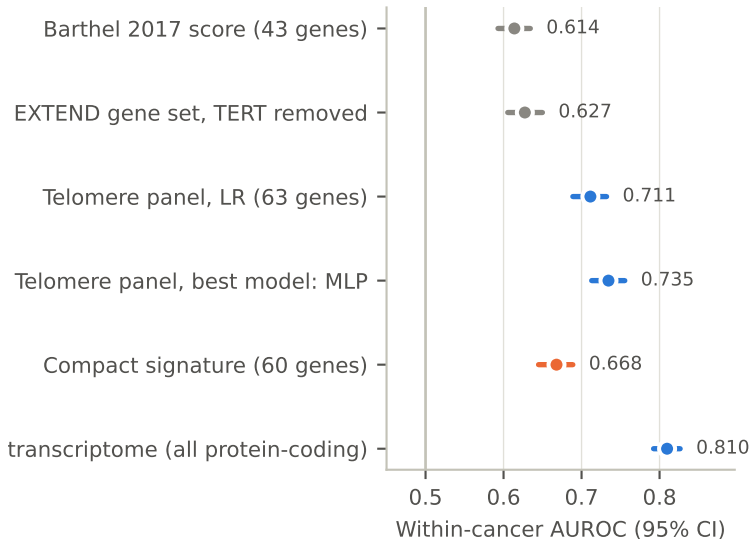
Telomerase activation (TERT excluded)
