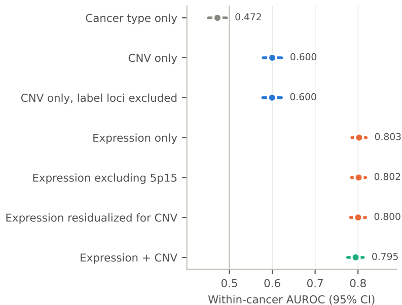
Telomerase activation (TERT excluded)
