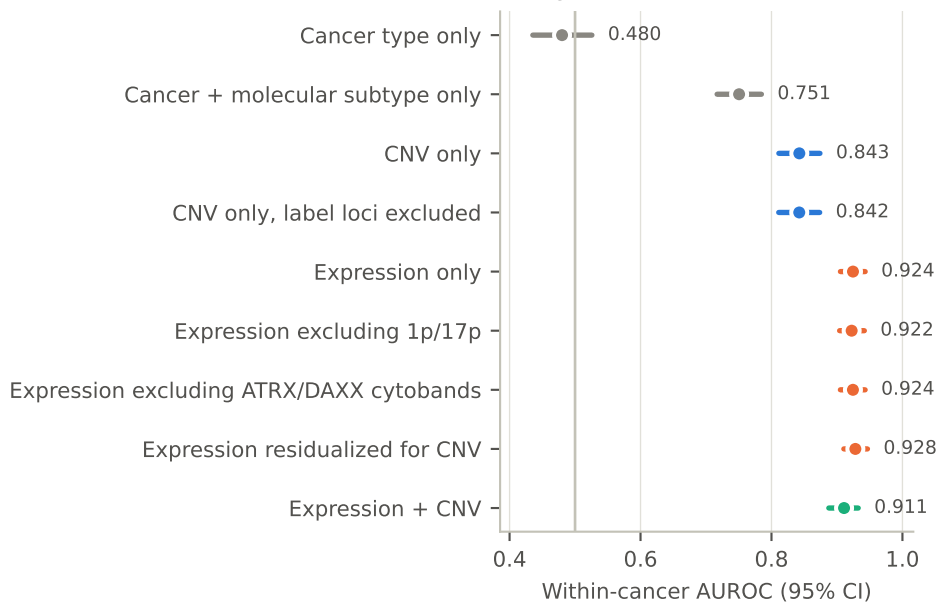
ALT, gliomas + sarcomas
