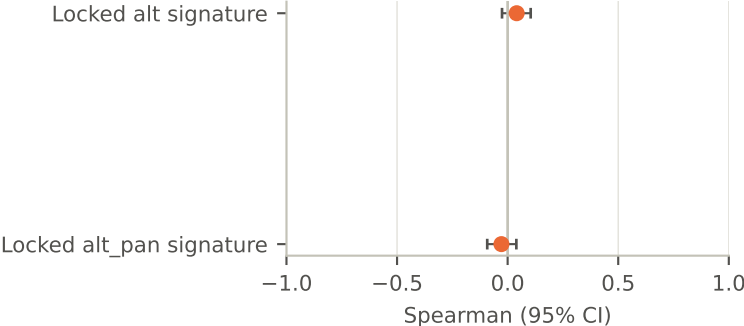
Correlation with C-circle abundance
