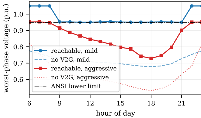
Fig. 2. Worst-phase voltage by hour with no V2G and under optimized per-hub dispatch. The mild-peak envelope clears the limit all day; eleven aggressive-peak hours cannot be cleared at any dispatch.
