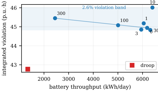
Fig. 5. Violation against battery throughput as the degradation weight is swept from 0 to 300 (labels). Violation stays inside a 2.6 percent band while throughput falls by sixty percent.
