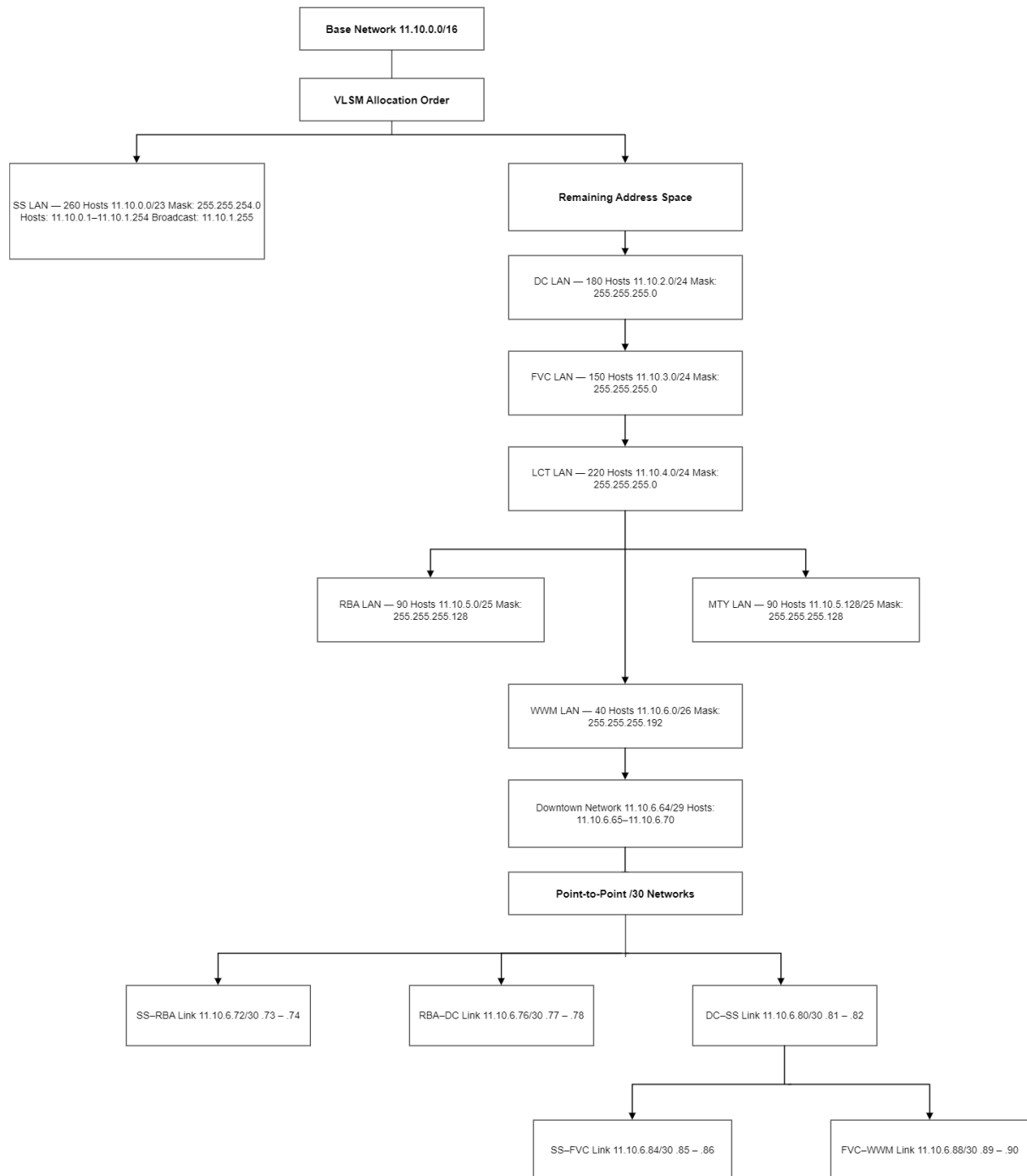
Figure 2: The complete VLSM allocation tree for the base network 11.10.0.0/16.
