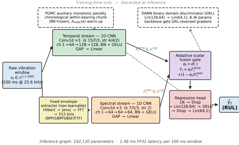
Figure 2: DSAFLite+PGMC architecture. Raw vibration drives a temporal 1D CNN and, in parallel, a fixed (non-learnable) Hilbert-envelope-spectrum extractor feeding a compact 3-layer 1D CNN; an adaptive scalar gate fuses the two 128-dimensional streams, and a regression head outputs RUL. The PGMC auxiliary monotonic penalty and the binary DANN domain discriminator (dashed) act only during training and are discarded at inference (192,130 parameters, 1.48 ms FP32 per 100 ms window).
