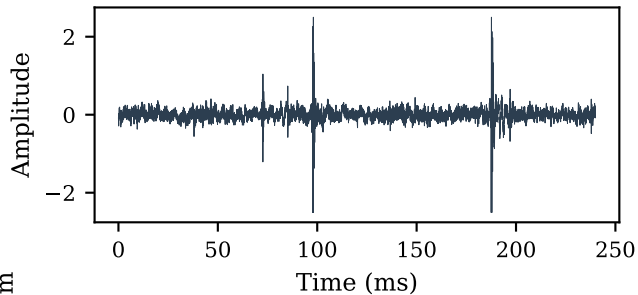
Inner-race fault, 600 rpm
