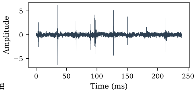
Inner-race fault, 1000 rpm
