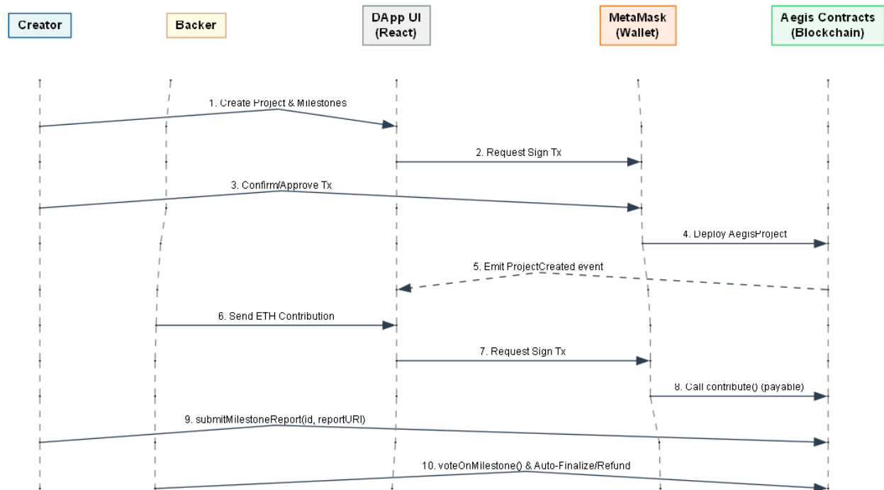
Figure 3: Sequence Diagram Interaksi UI-Wallet-Smart Contract
