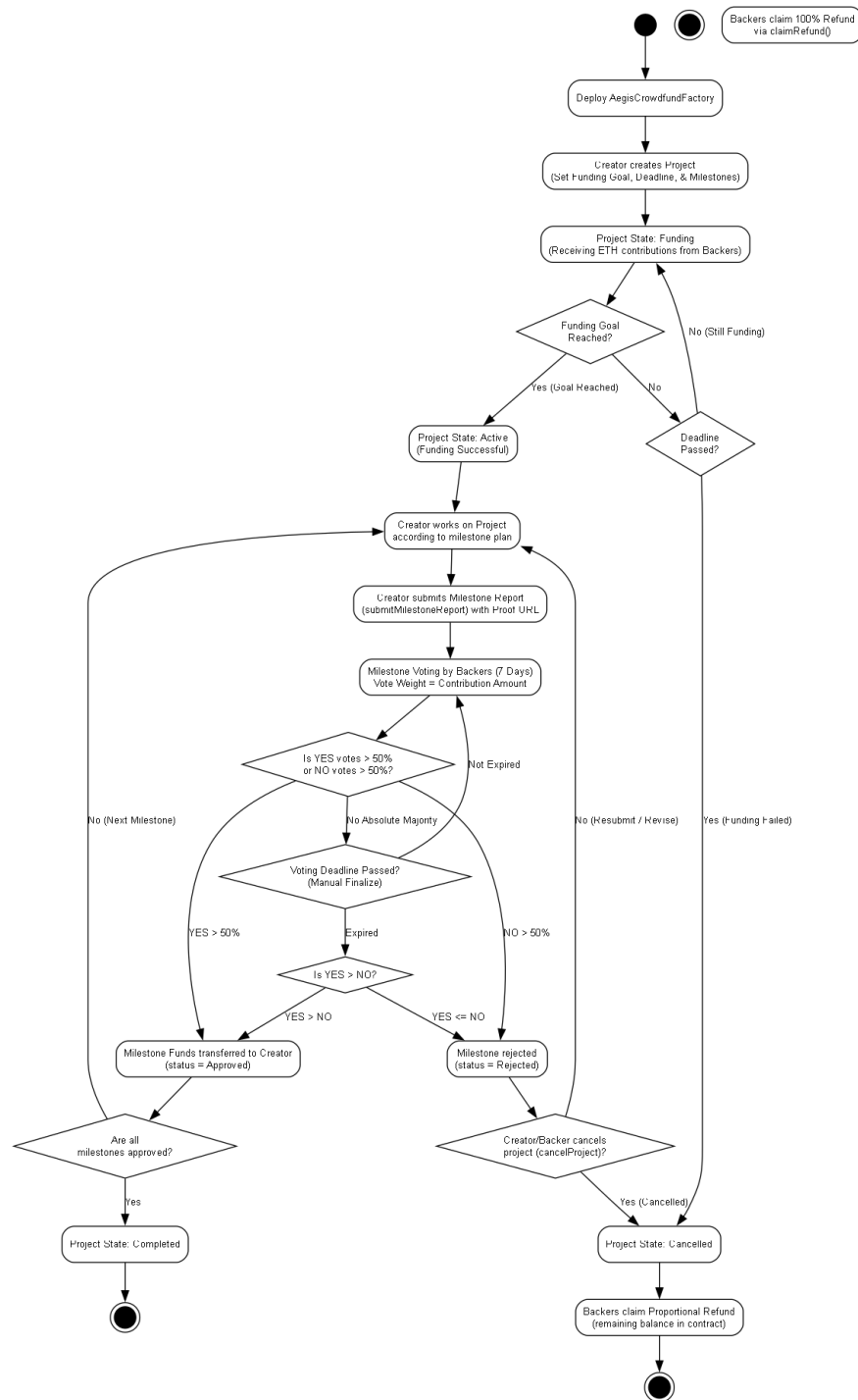
Figure 2: Activity Diagram Alur Crowdfunding
