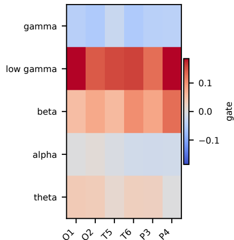
(e) SRM channel-band gate
