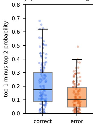
(b) Prediction margin
