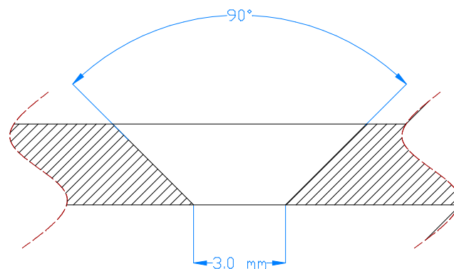
Hole detail
