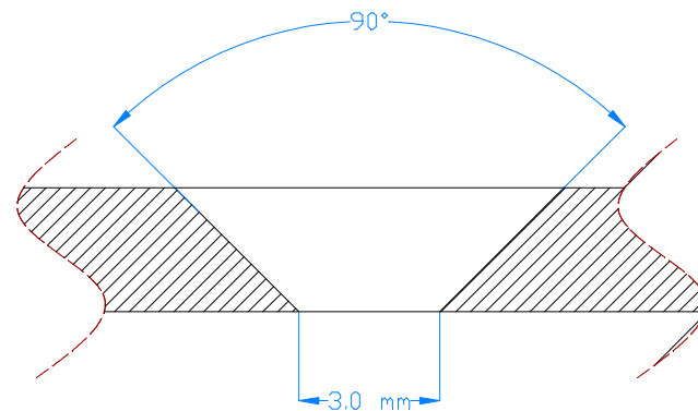
Hole detail
