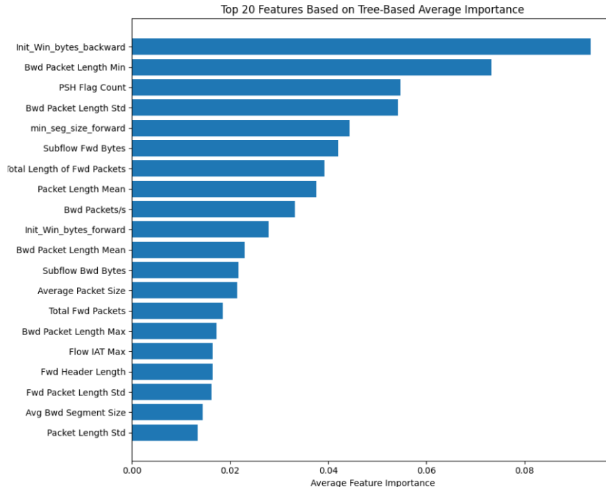
Figure 3: Top 20 feature importance scores.
