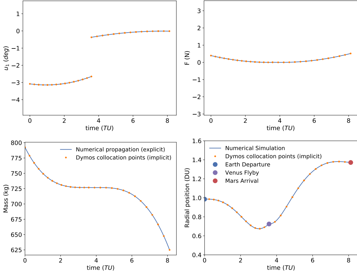
Fig. 6 Plots showing how the steering angle, thrust magnitude, spacecraft mass, and radial distance change over the trajectory with variable departure/arrival dates. Time is plotted in the Earth-Sun canonical time units.
