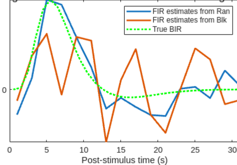
Fig 1.13. FIR estimates for Ran vs Blk designs
