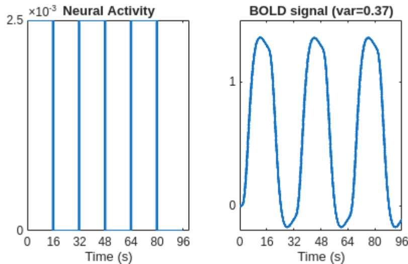
Fig 1.5. Blocked, Epoch Model, Block Length = 16
