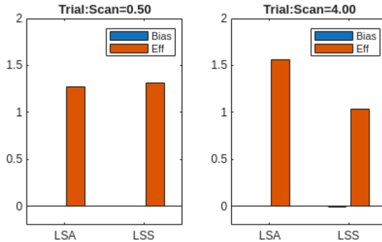
Fig 2.6. Efficiency and Bias for LSA versus LSS
