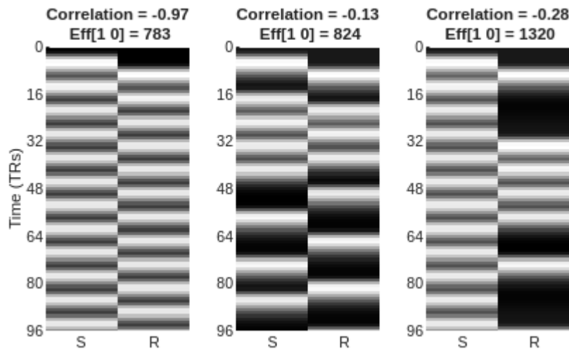
Fig 1.21. Separating Stimuli (S) and Responses (R)
