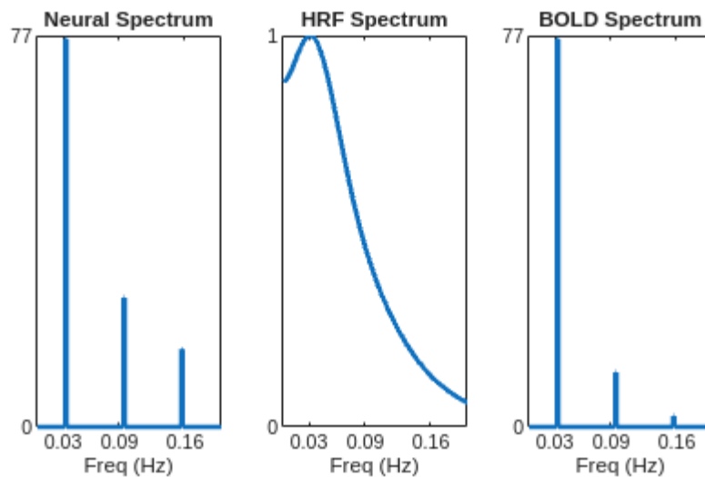
ig 1.6. Fourier Transform of Epoch Model, Block Length = 1
