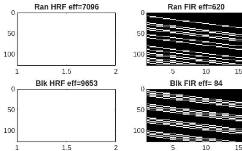
Fig 1.12. Detection Power vs Estimation Efficiency
