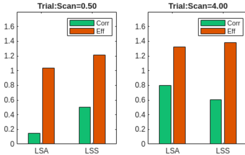
Fig 2.7. Trial-wise correlation for LSA versus LSS
