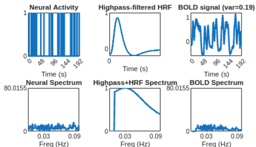
Fig 1.11. Randomised design (again), SOAmin = 4
