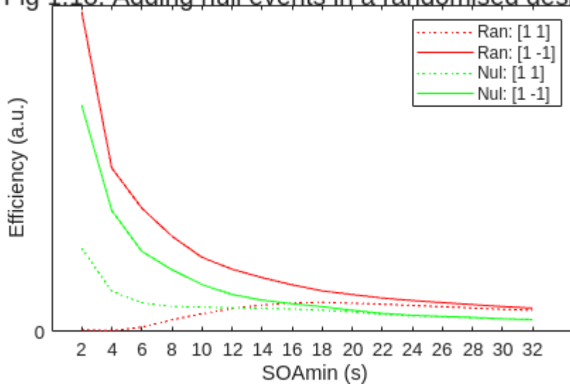
Fig 1.18. Adding null events in a randomised design
