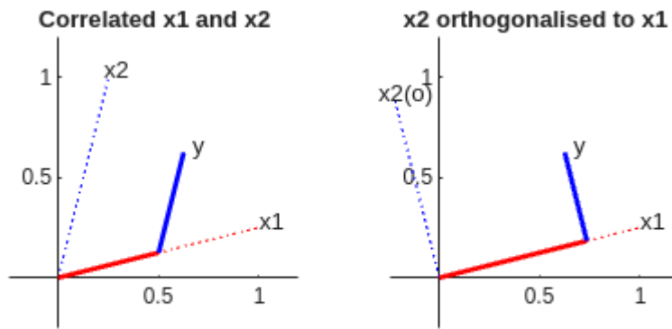
Fig 1.20. Geometric perspective on orthogonalisation
