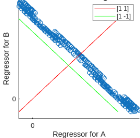
Fig 1.19. Correlation between regressors, R = -0.99
