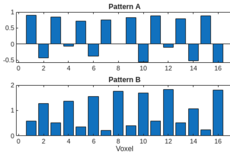
Fig 3.1 Mean estimated pattern across trials
