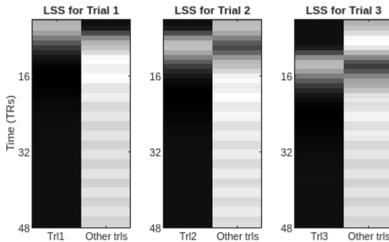
Fig 2.5. Example LSS design matrices
