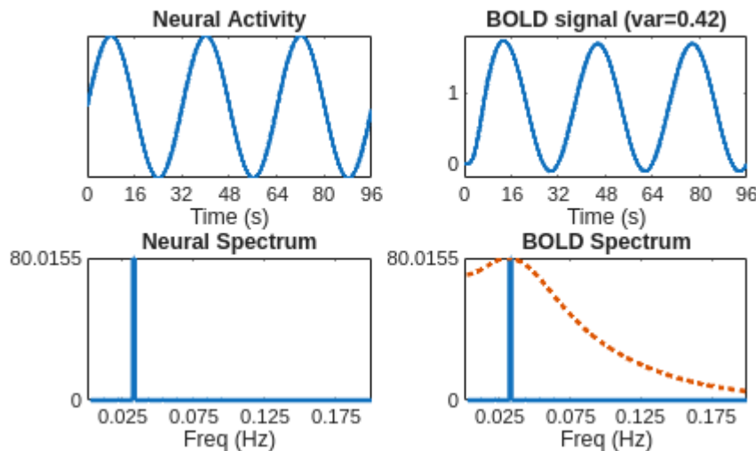
Fig 1.7. Fourier Transform of Optimal Sinusoidal Design
