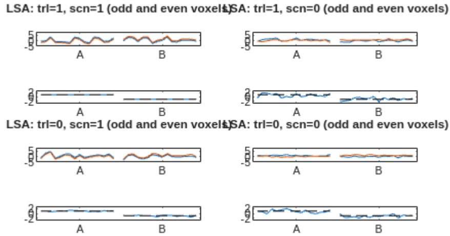
Fig 3.4. Spatial covariation of trial vs scan variability with LS.
