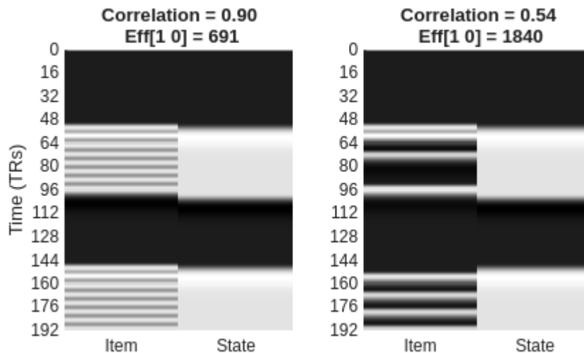
Fig 22. Separating state vs item effects
