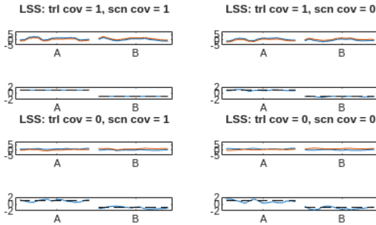
Fig 3.4. Spatial covariation of trial vs scan variability with LS.
