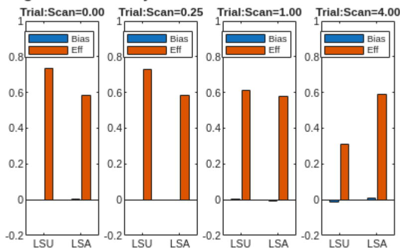
Fig 2.2. Efficiency and Bias for LSA versus LSU
