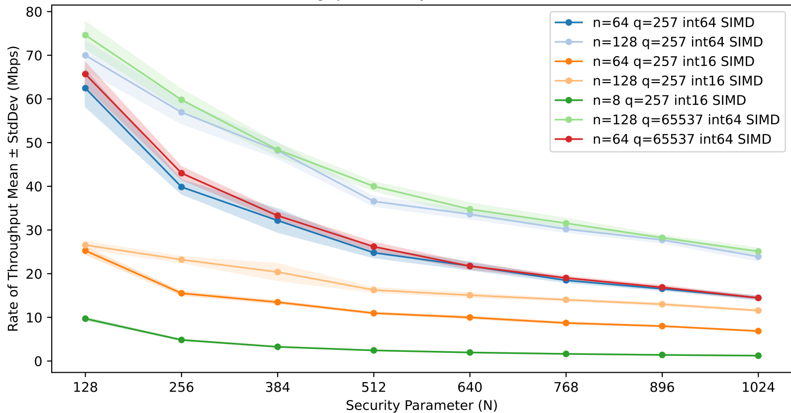
MiNTT Throughput Rate by Parameterization (SIMD)
