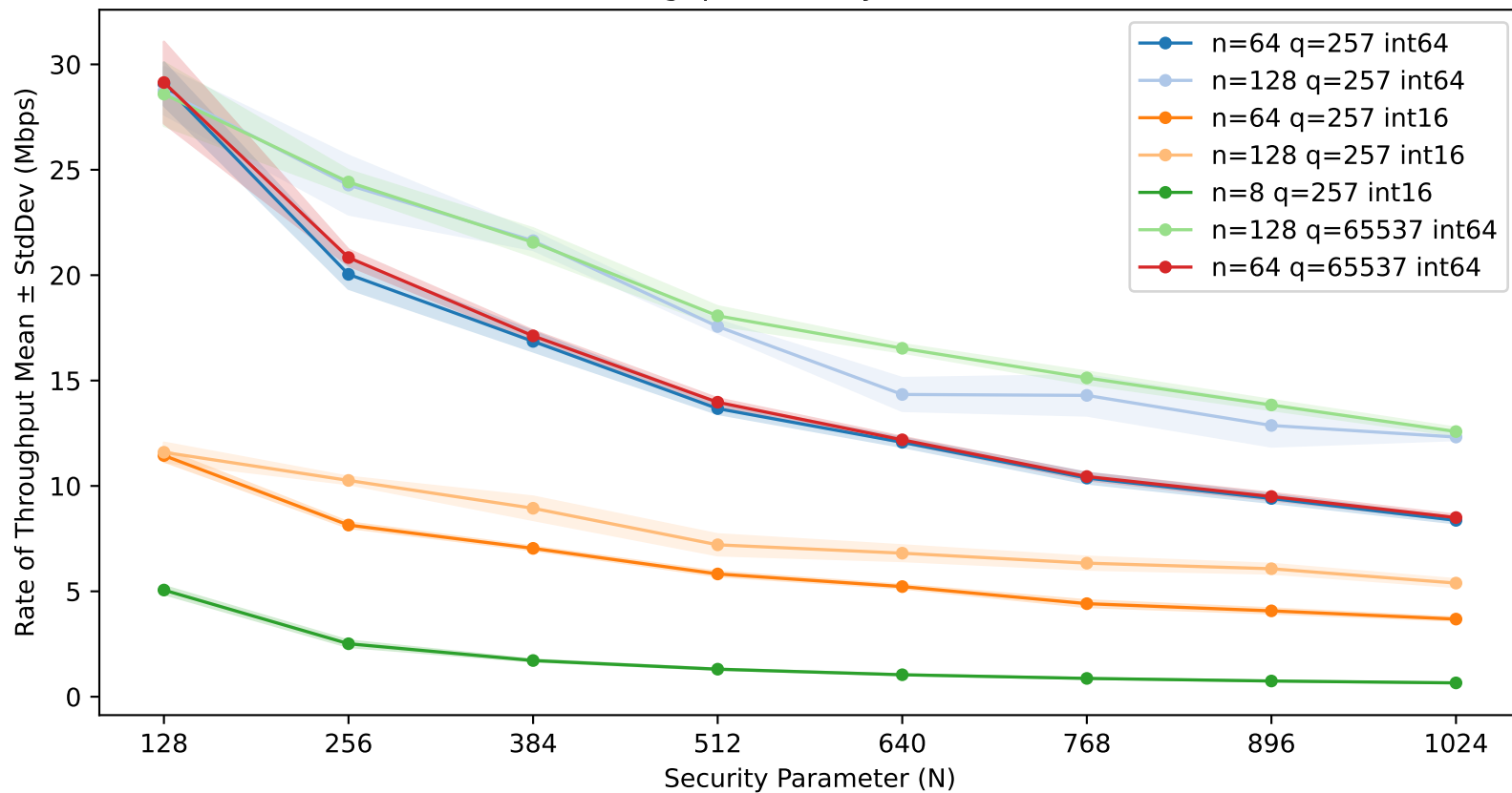
MiNTT Throughput Rate by Parameterization
