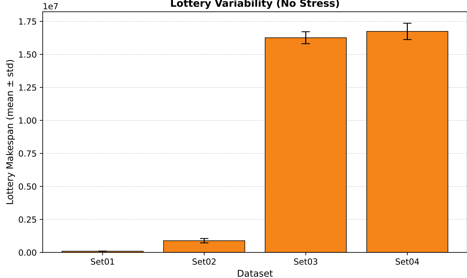
Lottery Variability (No Stress)
