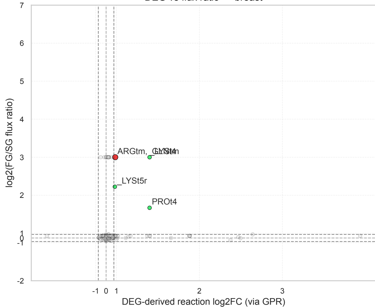
DEG vs flux ratio — breast
