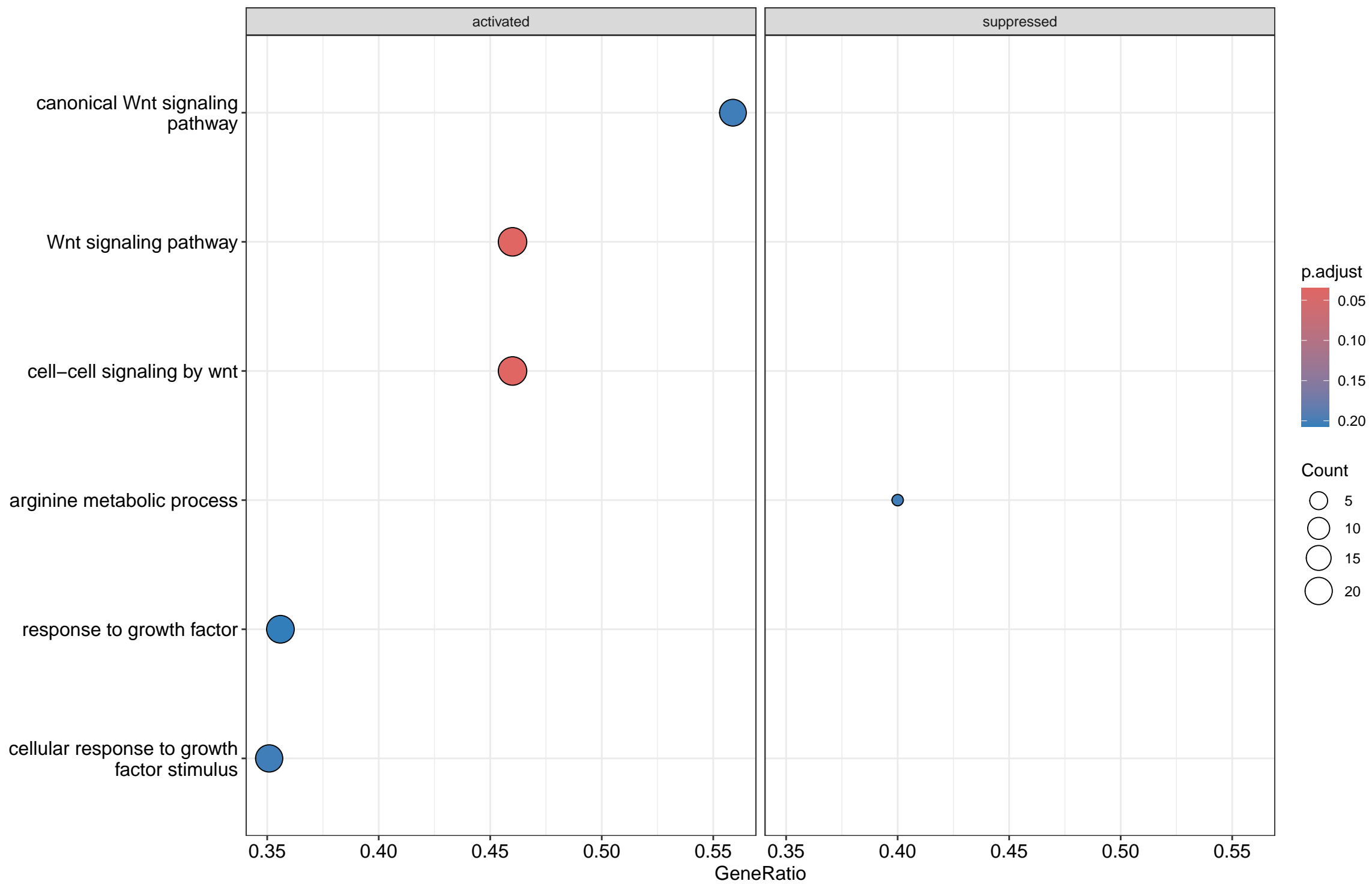
Dotplot – liver
