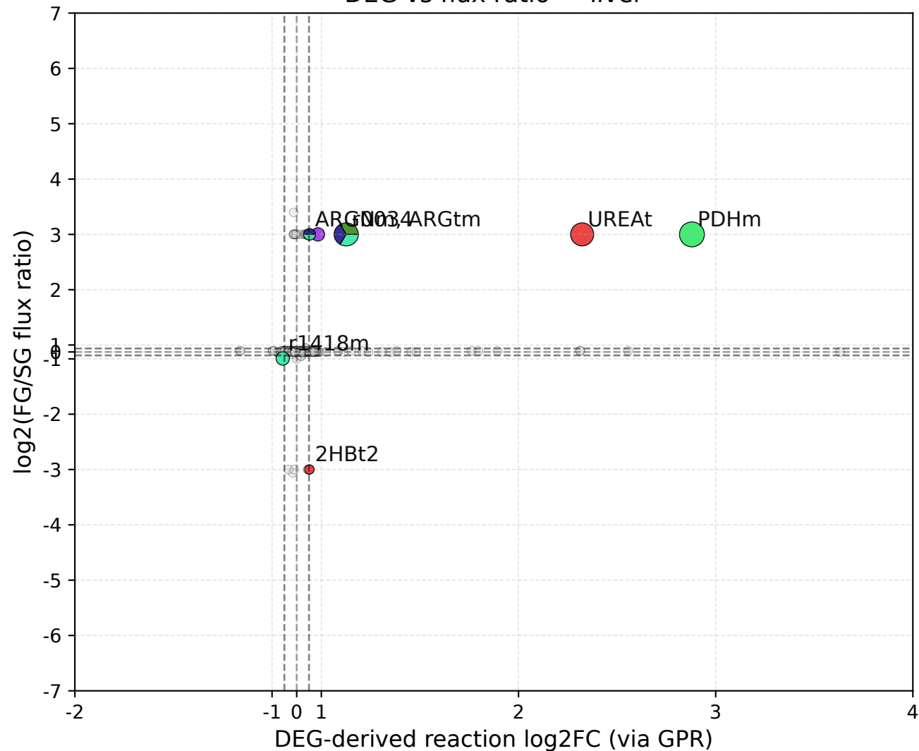
DEG vs flux ratio — liver
