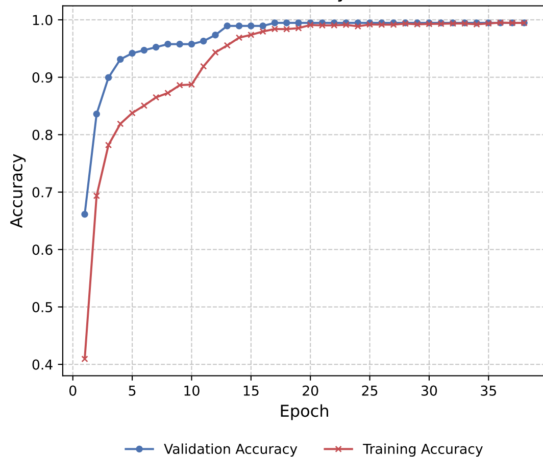
Accuracy
