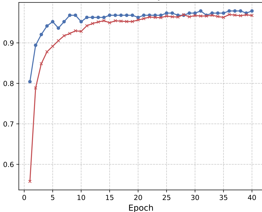
Accuracy
