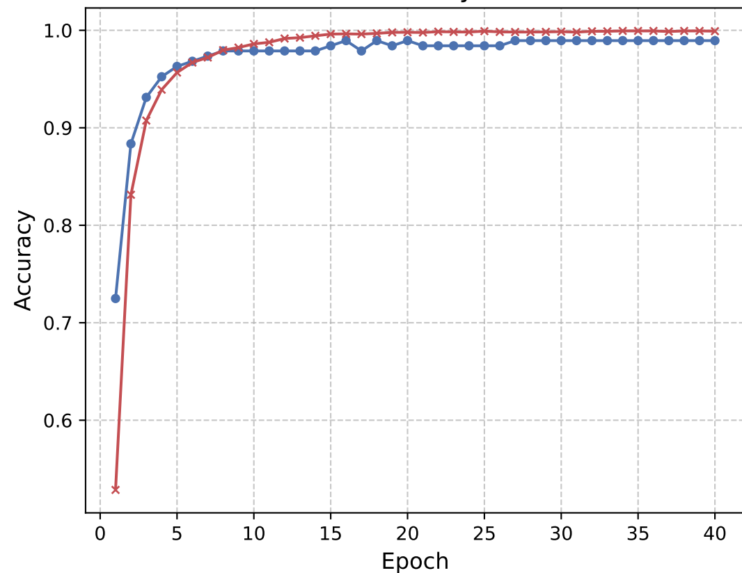
Accuracy
